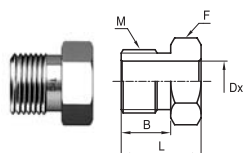
HMFS Male Nut
