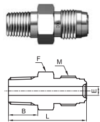
Male Connector(NPT)
