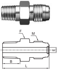
Male Connector(PT)
