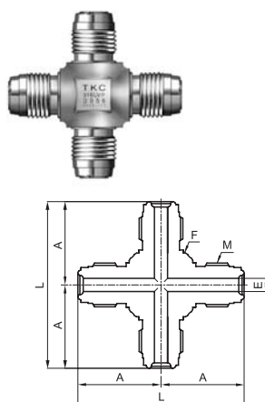
Union Cross
