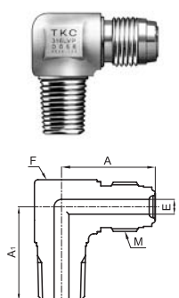
Male Elbow (NPT)
