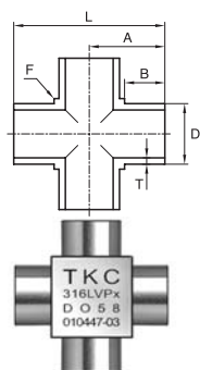
Micro Cross
