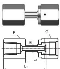
Welded Female Connector(PT)
