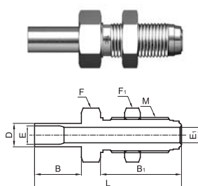
HMFS Bulkhead Connector
