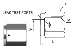
HMFS Female Nut
