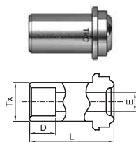
Socket Weld Short Gland
