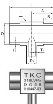
Micro Reducing Tee
