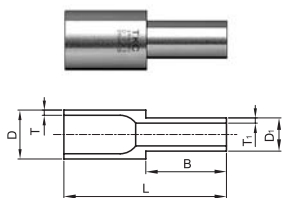
Reducer
