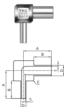
Reducing 90° Elbow
