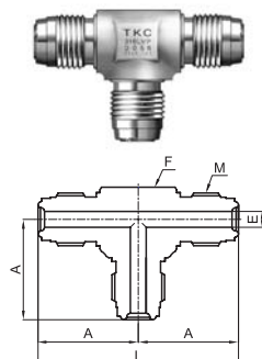
Union Tee
