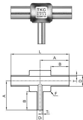
Reducing Tee
