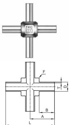
Cross Tee
