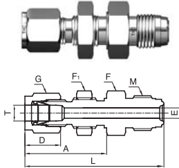
Tube Fitting Bulkhead Connector
