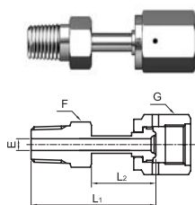
Welded Male Connector(PT)
