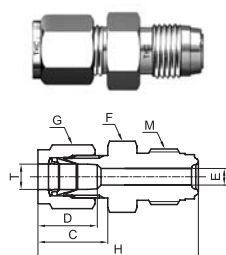
Tube Fitting Connector
