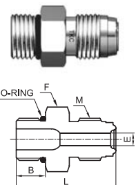
Male Connector(ST)
