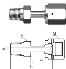
Welded Male Connector(NPT)
