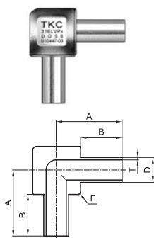
90° Elbow
