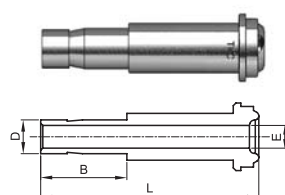
Tube Adapter
