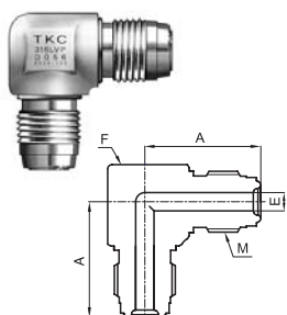
Union Elbow
