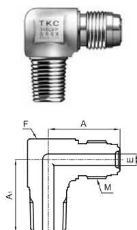
Male Elbow (PT)
