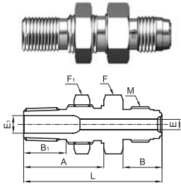
Male Bulkhead Connector(NPT)
