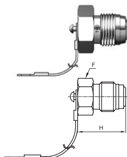
Plug (Cable Type)
