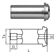
Socket Weld Reducing Long Gland
